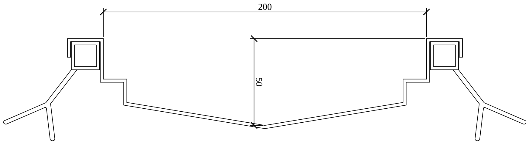
Typical Channel Section,
